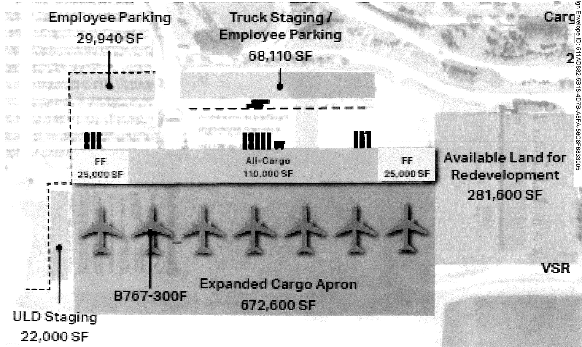
Figure 6.17: Ultimate Cargo Facility Plan Source: AECOM (2015)
